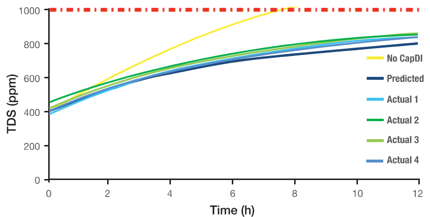
TDS VS. LAUNDERING TIME
